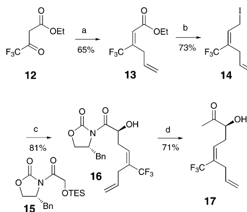
Scheme 2. Synthesis of the alkyl sector 17 . Reagents and conditions: a) 1. Allyl bromide, In, THF/H 2 O (3:1), 48 °C, 85%; 2. SOCl 2 , pyridine, 55 °C, 77%; b) 1. DIBAL-H, CH 2 Cl 2 , –78 °C → RT, 99%; 2. I 2 , PPh 3 , imidazole, CH 2 Cl 2 , 74%; c) 1. LiHMDS, THF, –78 °C → RT; 2. HOAc/THF/H 2 O (3:1:1), 81% for two steps; d) 1. AlMe 3 , MeONHMe, THF, 0 °C → RT, 97%; 2. MeMgBr, THF, 0 °C, 53% (73% based on recovered starting material). DIBAL-H = diisobutylaluminum hydride, HMDS = hexamethyldisilazide.
