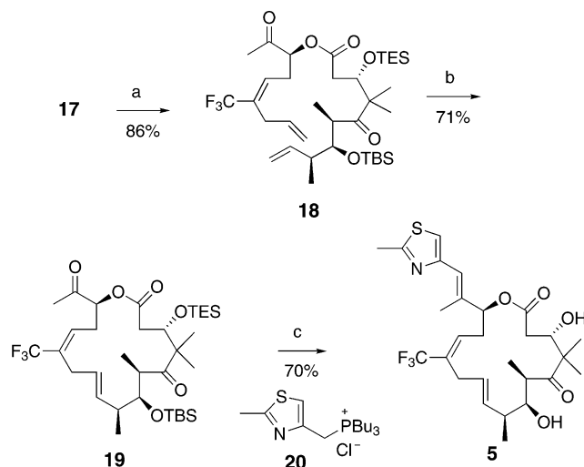
Scheme 3. Final steps of the synthesis of 5 . Reagents and conditions: a) EDCI, DMAP, CH 2 Cl 2 , 11 , 0 °C → RT, 86 % based on 11 ; b) second-generation Grubbs catalyst, toluene, 110 °C, 20 min, 71 %; c) 1. KHMDS, 20 , THF, –78 °C → –20 °C, 70 %; 2. HF-pyridine, THF, 98 %. EDCI = 1-[3-(dimethylamino)propyl]-3-ethylcarbodiimide hydrochloride, DMAP = 4-(dimethylamino)pyridine.
